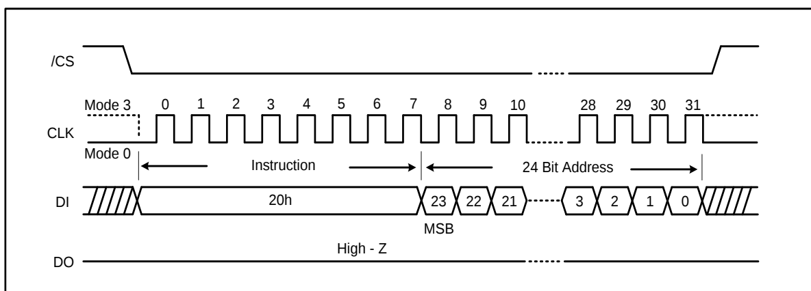
Figure 22a. Sector Erase Instruction (SPI Mode)
