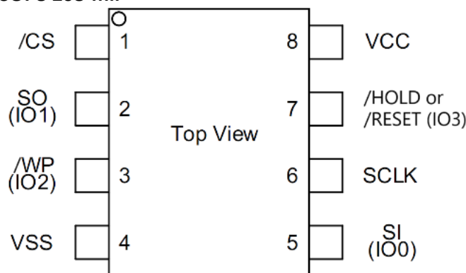
Figure 1a. 8-pin SOP 208-mil
