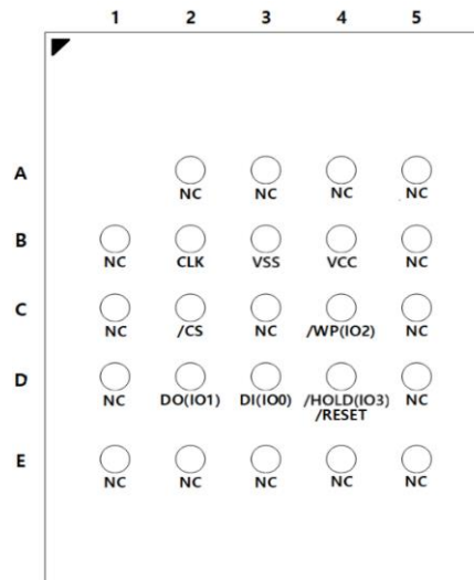
Figure 1d. 24-ball FBGA(Top View)
