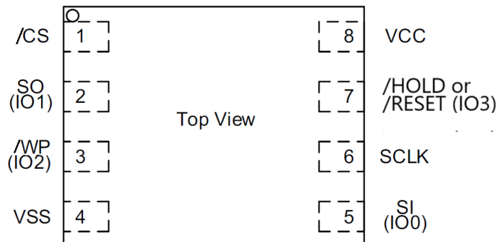
Figure 1c. 8-pad WSON 6x5/8x6-mm
