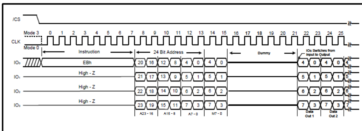
Figure 15a. Fast Read Quad I/O Instruction (Initial instruction or previous M5-4 ≠ 10, SPI Mode)
