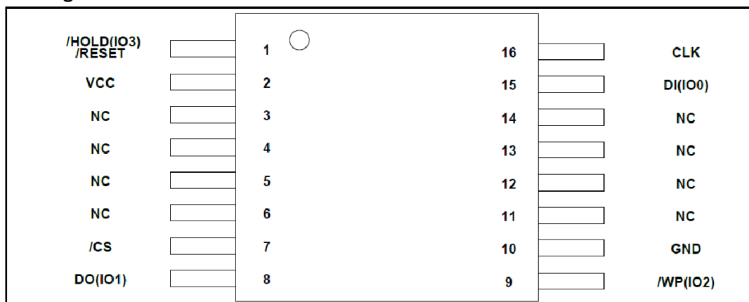
Figure 1b. 16-pin SOP 300-mil
